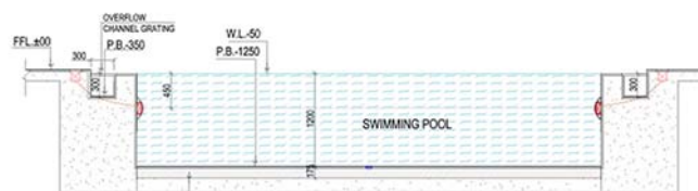
SECTION-X X
