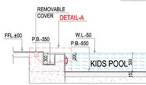
SECTION-Y
